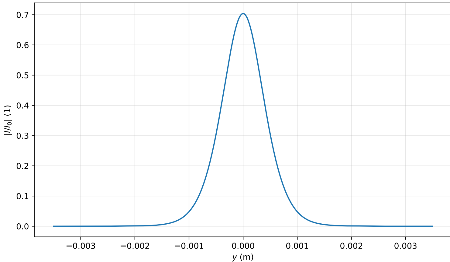
Intensity profile I(x=0, y, z=3.582)/I_0 , P_{in}=0.7P_{cr} , artificial time
